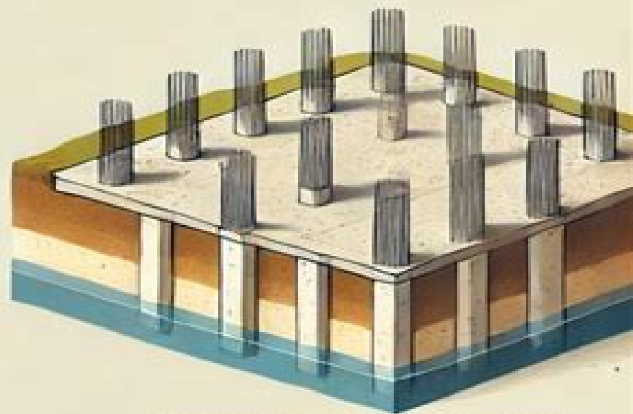
PILE FOUNDATION
