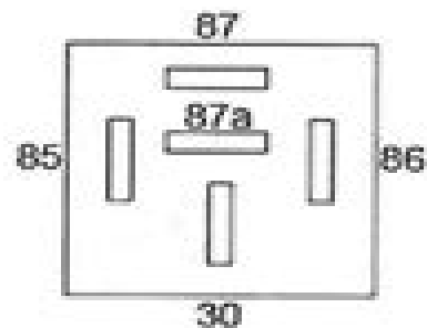
Detail of relay SOCKET Numbering
