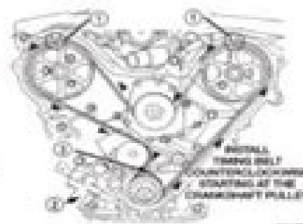
Fig. 99 Timing Belt—Installation
