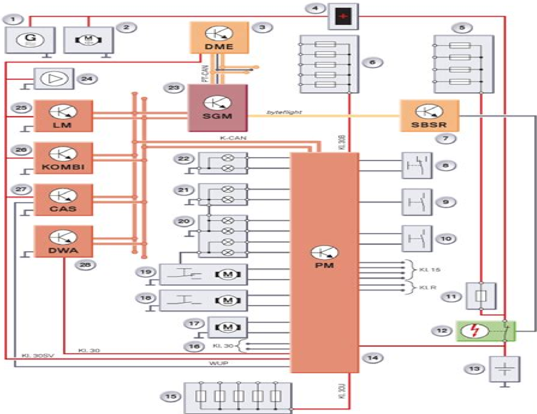
1 - System circuit diagram of the power supply in the E65/E66
