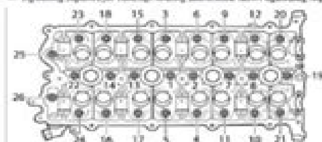
Fig. 20. Tightening sequence for camshaft housing Courtesy of PORSCHE OF NORTH AMERICA, INC.
