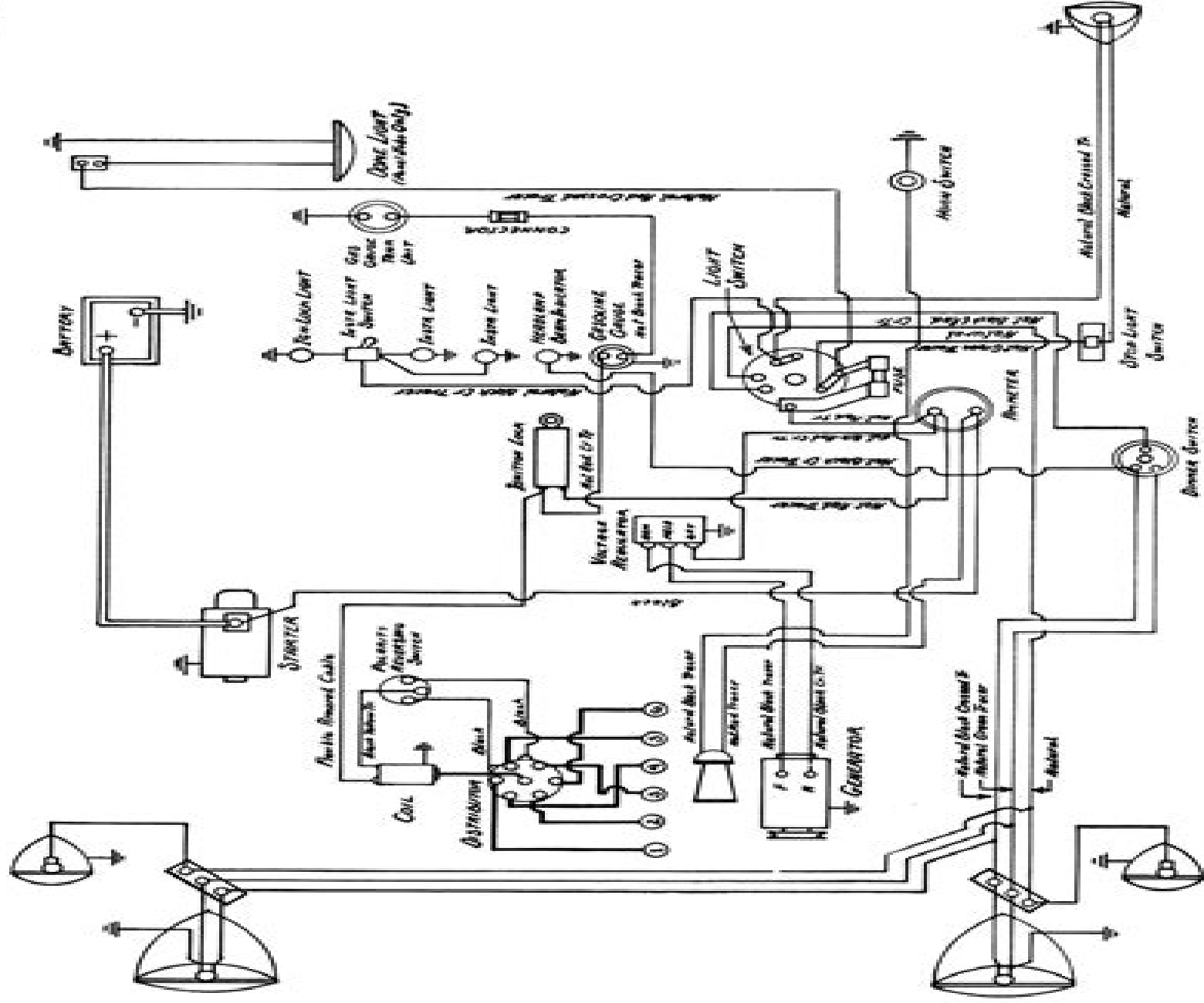
Fig. 46—Passenger Car Wiring Diagram
