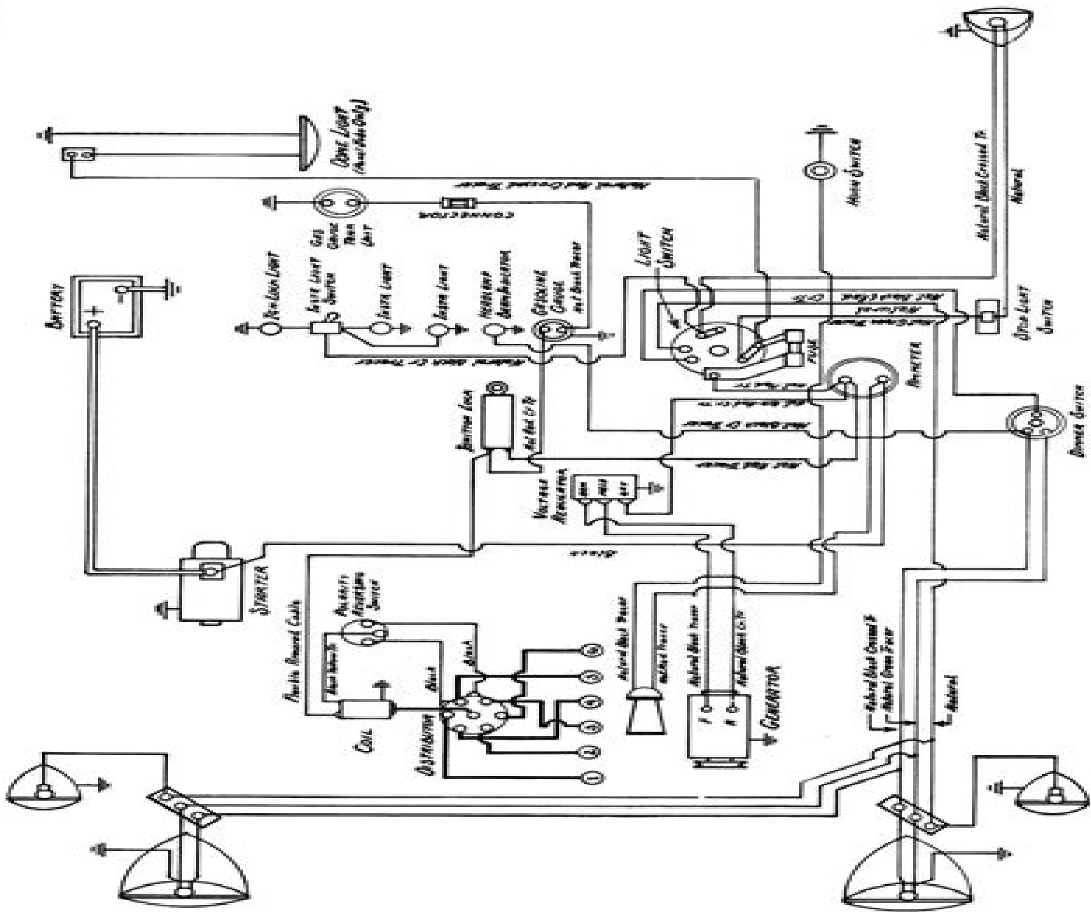
Fig. 60—Passenger Car Wiring Diagram 1941
