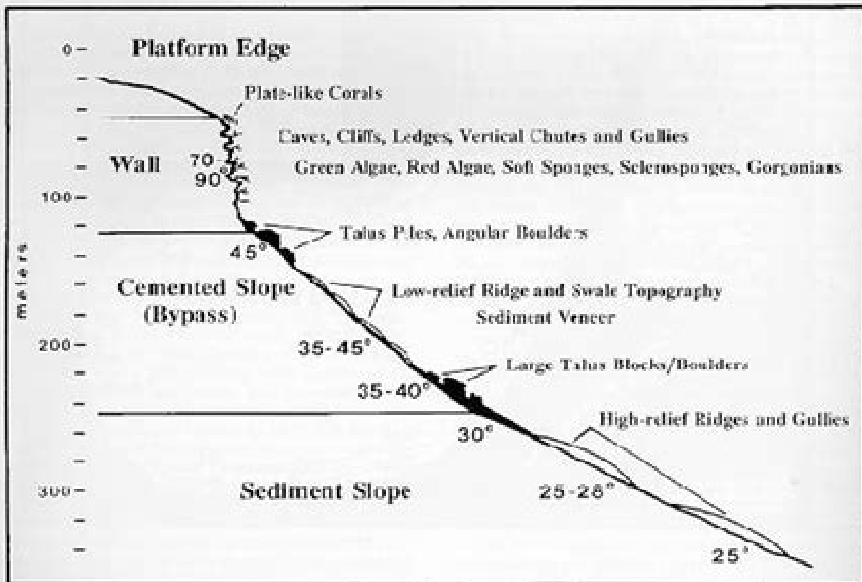
Figure 2. Representative profile of upper slope environments around the cul-de-sac of the Tongue of the Ocean. Profile was constructed from a synthesis of data accumulated during a total of 134 dives during 1987, 1988, and 1990. No vertical exaggeration. Modified from Grammer and Ginsburg (1992).
