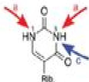
pseudouridine \psi
