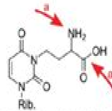
3-(3-amino-3-carboxypropyl)uridine acp^3U
