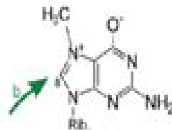
7-methylguanosine m^7G
