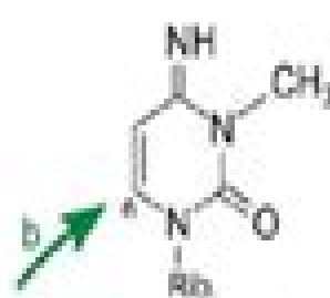
3-methylcytidine m^3C
