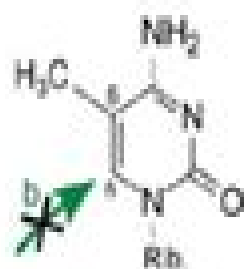
5-methylcytidine m^5C
