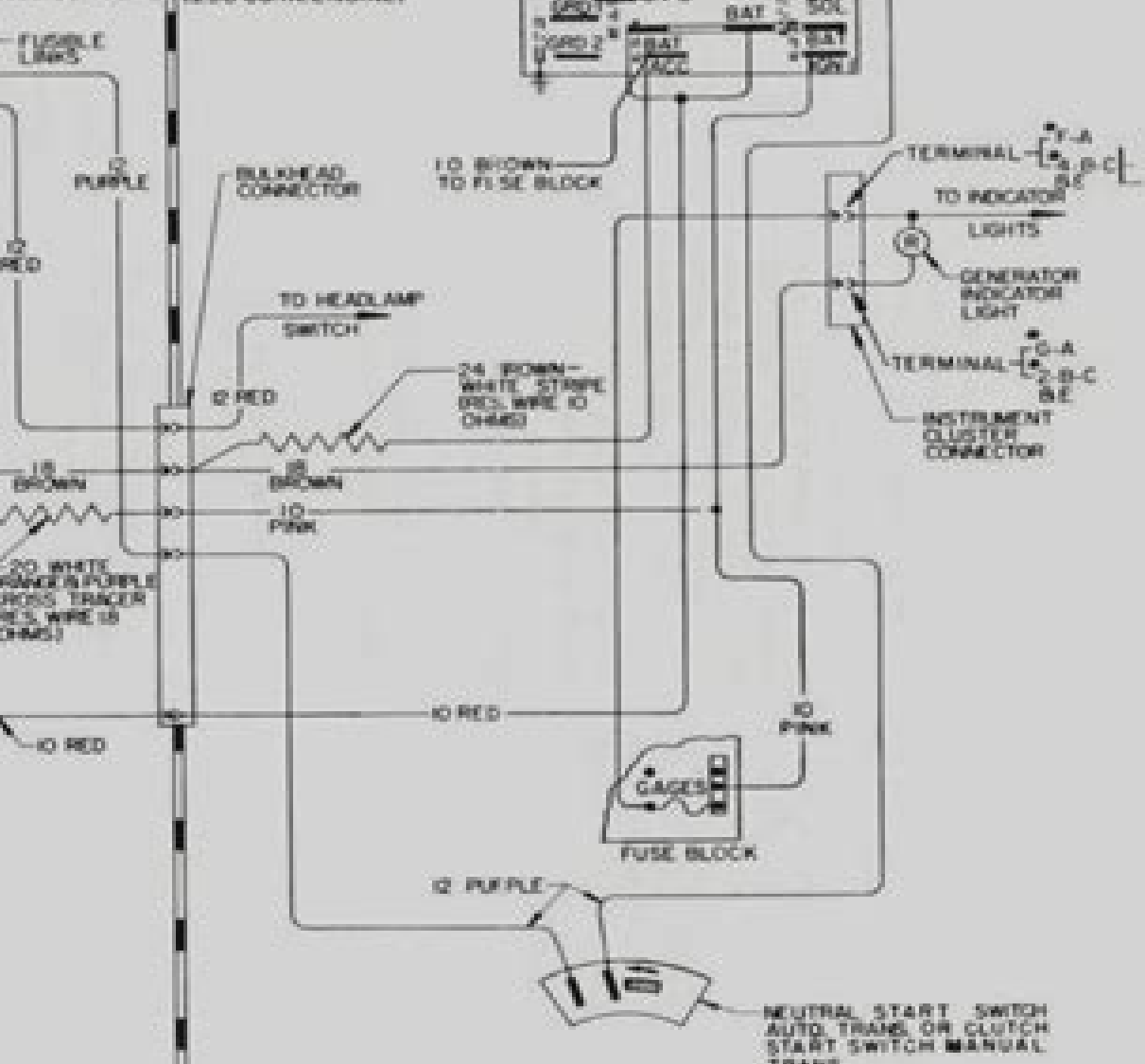
PART OF INSTRUMENT PANEL WIRING HARNESS
