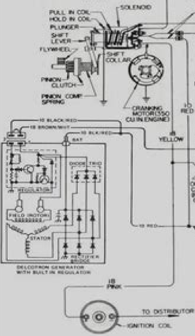
PART OF ENGINE WIRING HARNESS
