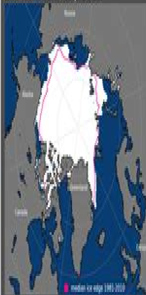
Sea Ice Extent, Sep 1980
