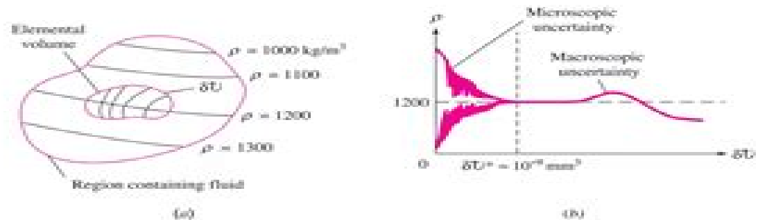
Fig. 1.4 The limit definition of continuum fluid density: (a) an elemental volume in a fluid region of variable continuum density; (b) calculated density versus size of the elemental volume.
