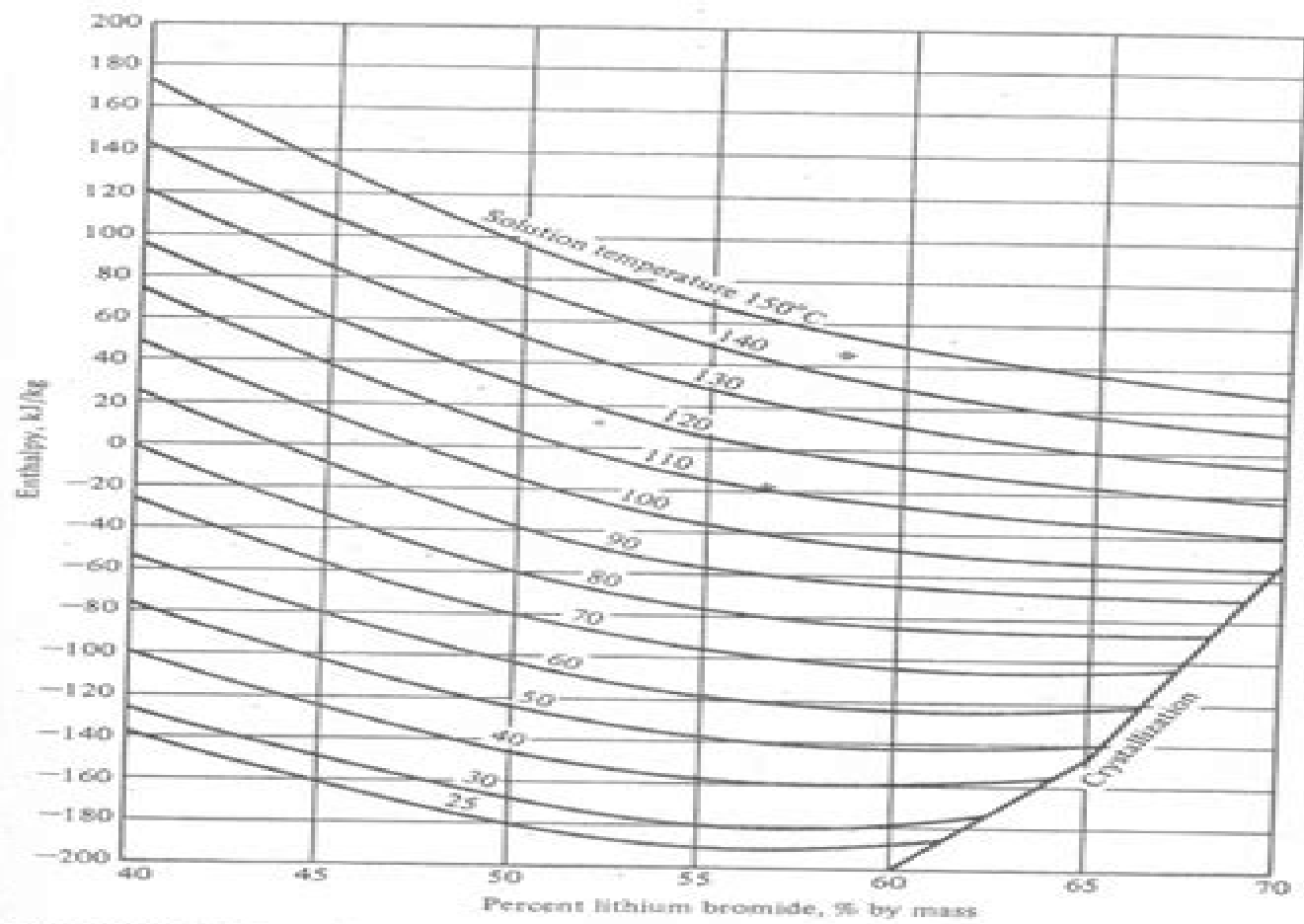
Figure 17-8 Enthalpy of LiBr-water solutions; data from Ref. 1.
