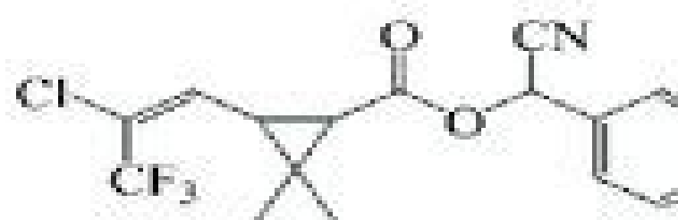
Lambda-cyhalo
