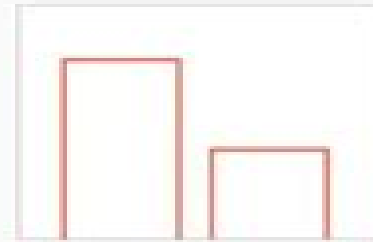
Bernoulli distribution
