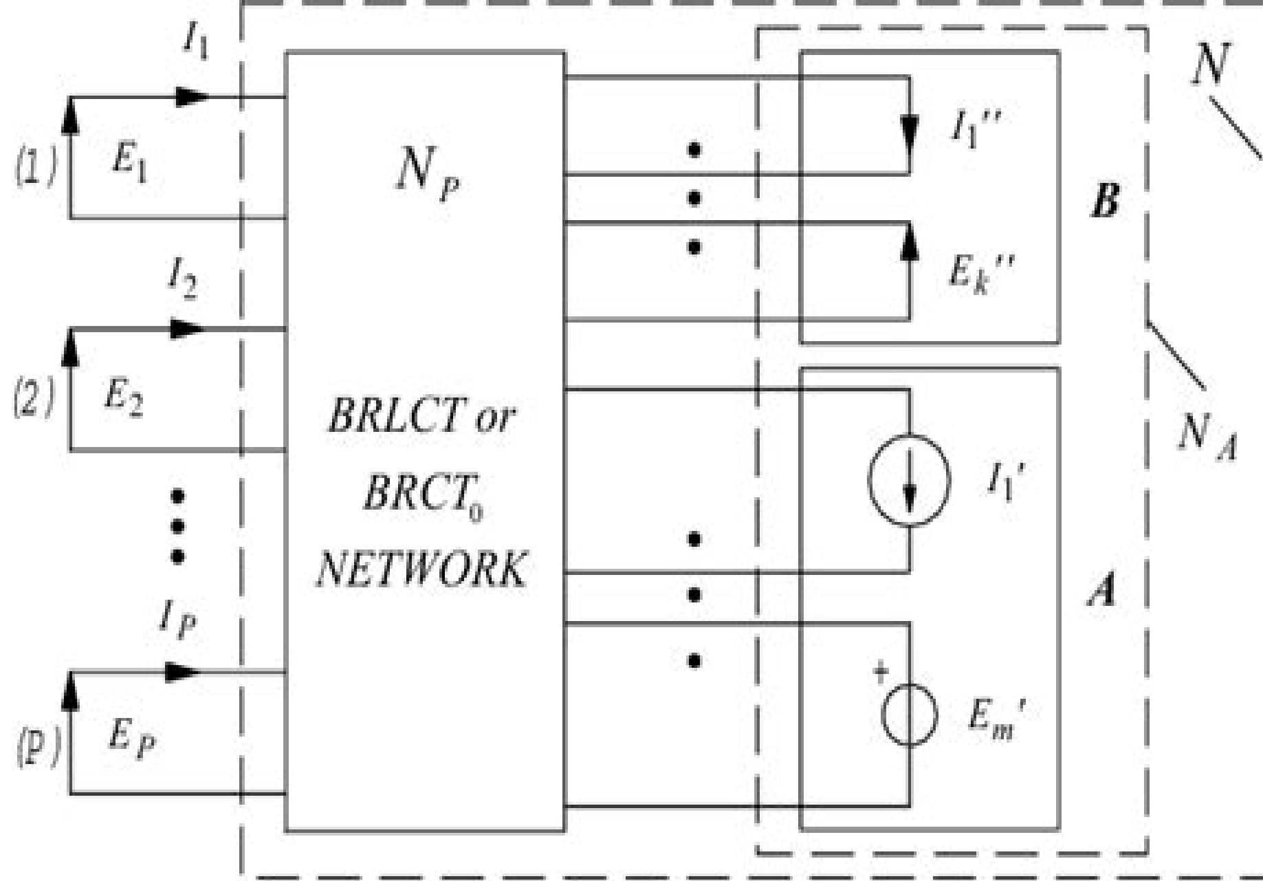
Figure 1. General active realization network
