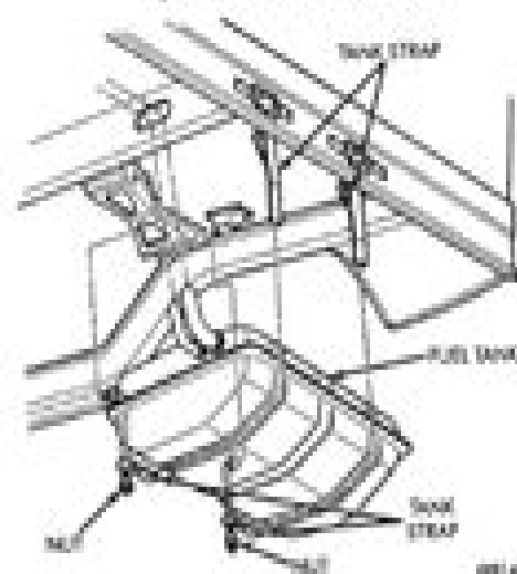
Fig. 3 Fuel Tank Remove/Install—KJ Models
