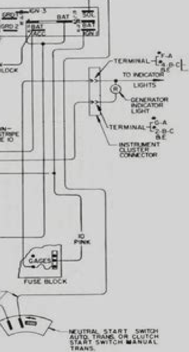
PART OF INSTRUMENT PANEL WIRING HARNESS
