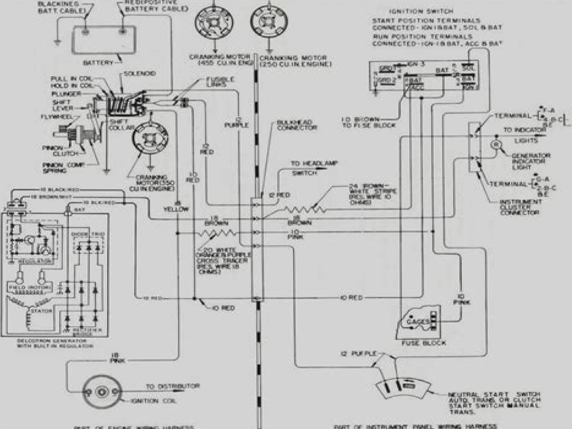
PART OF ENGINE WIRING HARNESS
