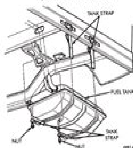
Fig. 3 Fuel Tank Removal/Install—XJ Models
