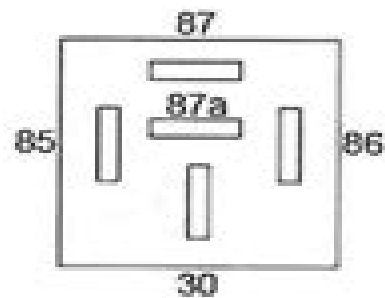
Detail of relay SOCKET Numbering
