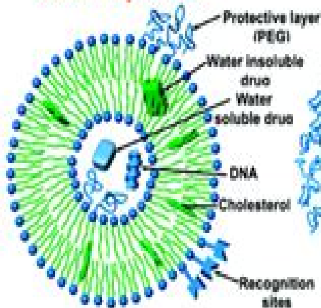
Stealth Liposome
