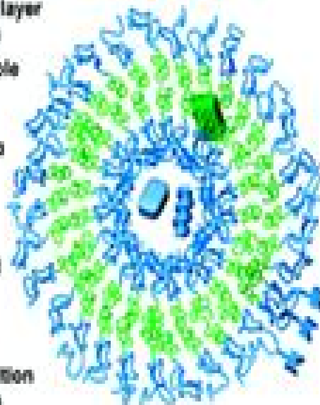
Polymersome
