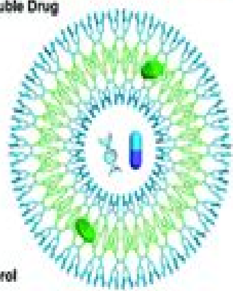
Glycodendrimersomes
