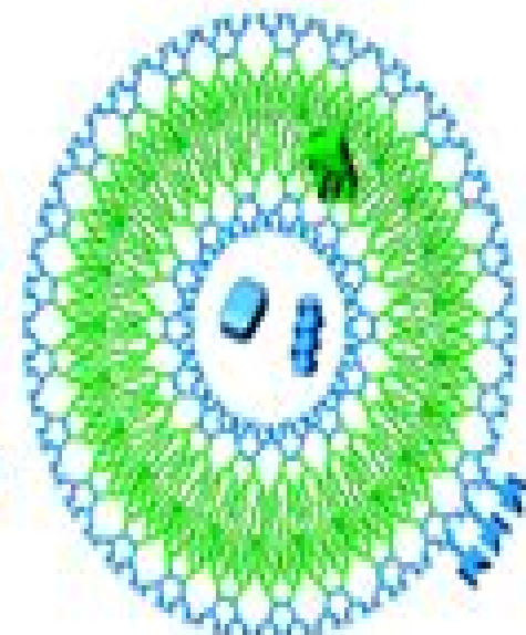
Dendrimersome
