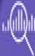
Time Series Models
