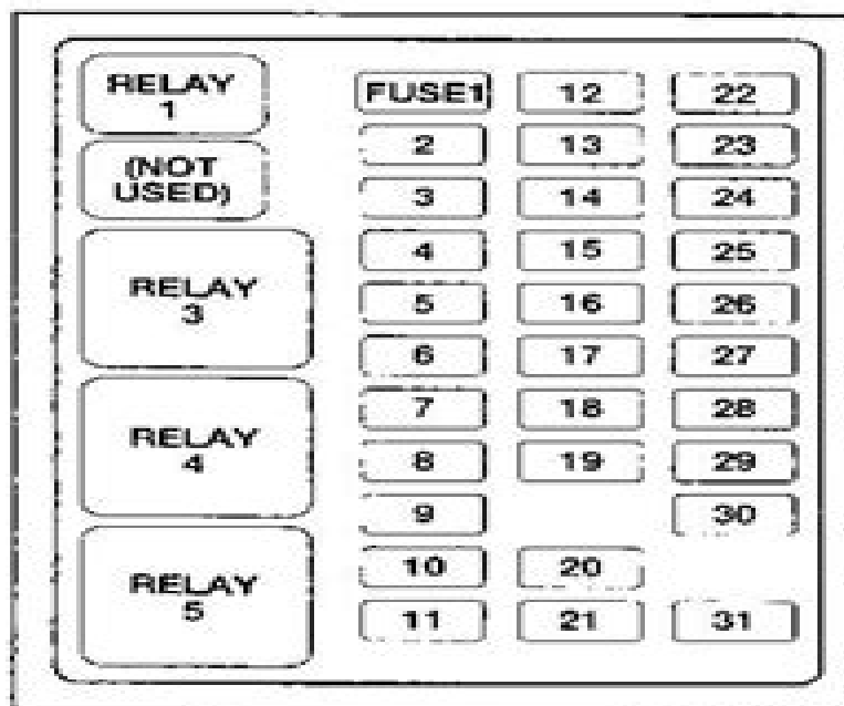
Fig. 3: Central Junction Box Legend (1 Of 3)
