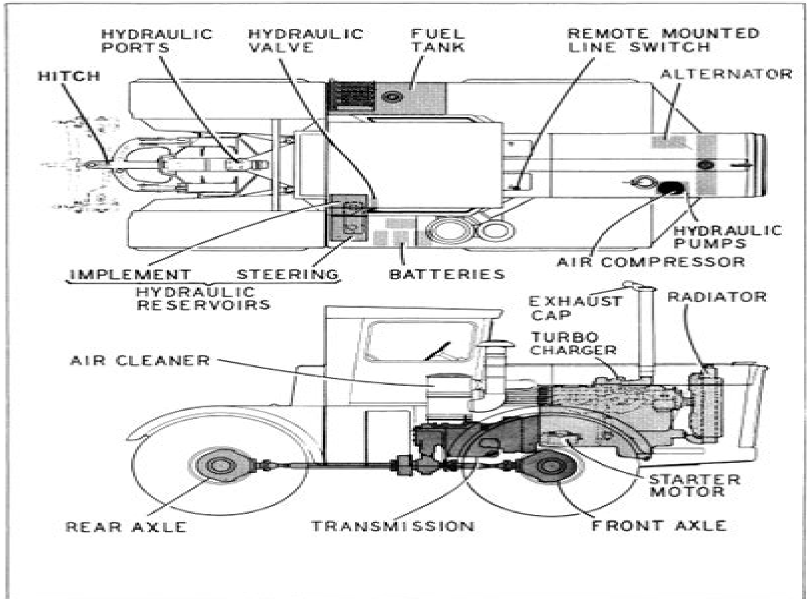
Figure 5. General arrangement
