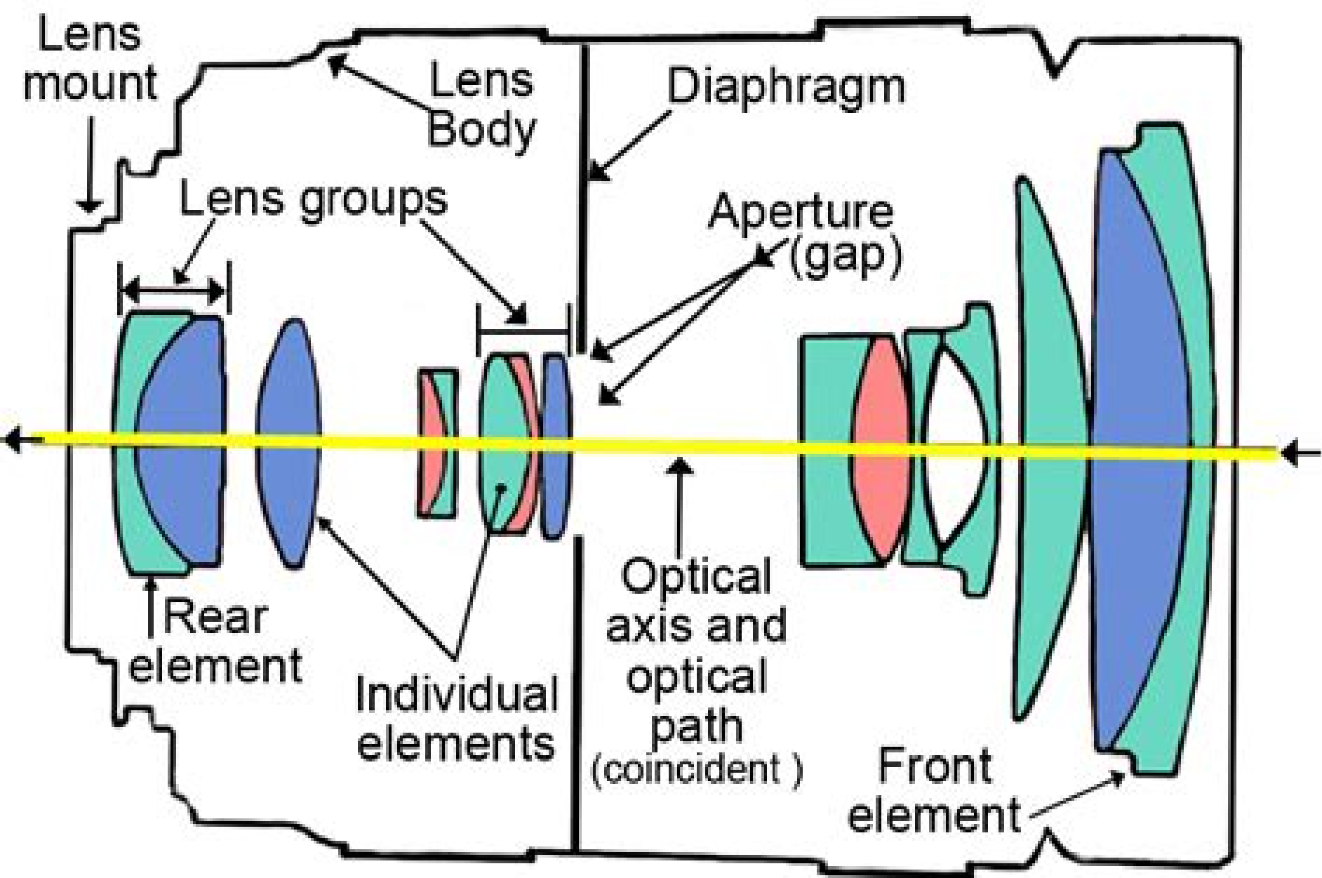
Generalised photographic lens
