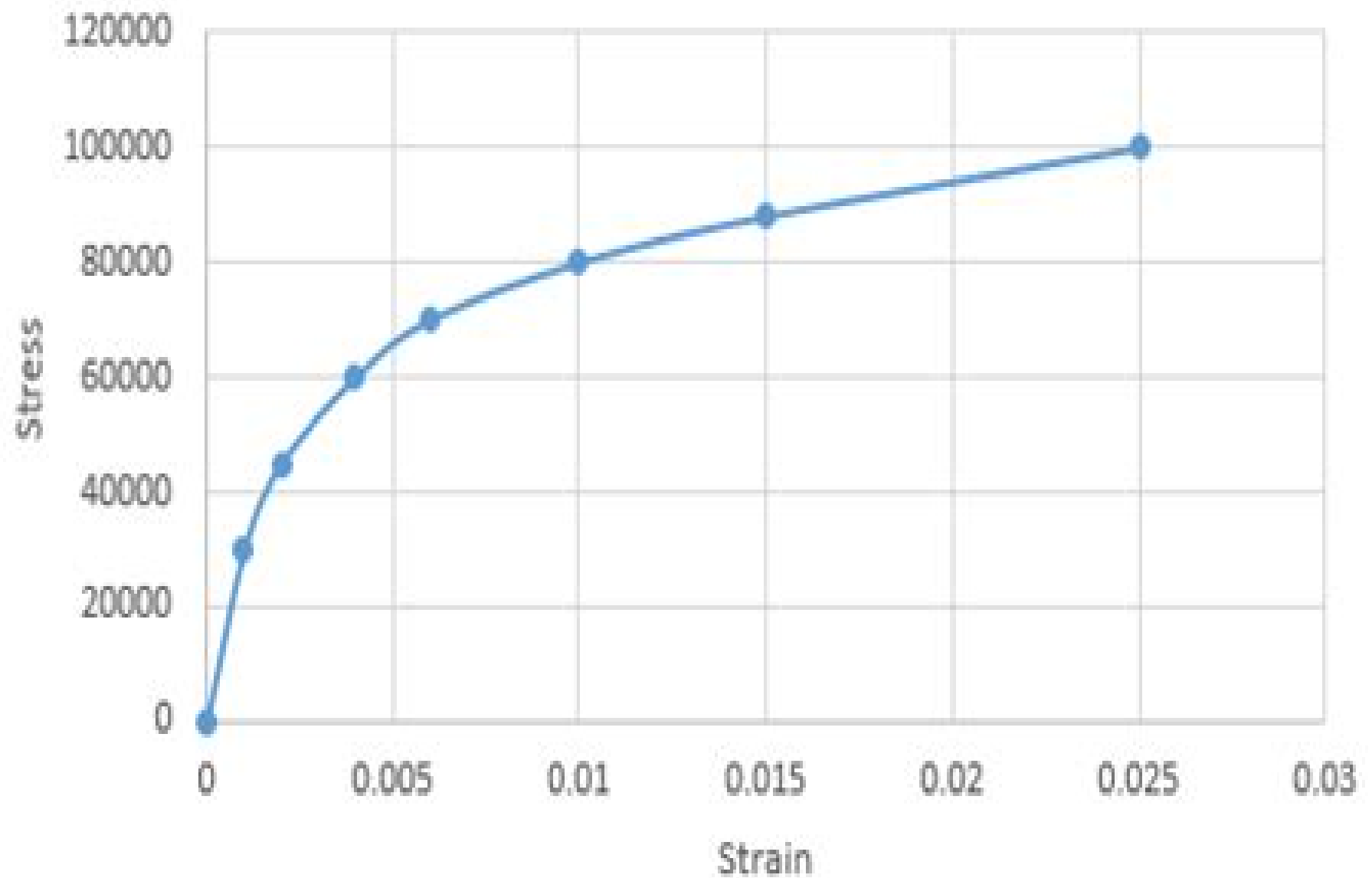
Measured Stress-Strain Curve
