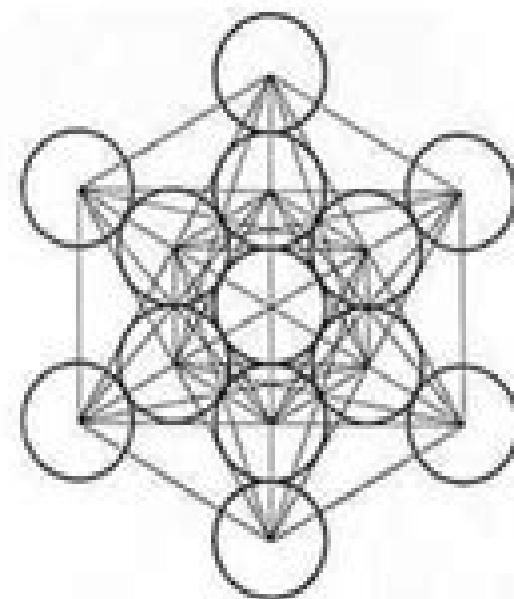
Metatron's Cube
