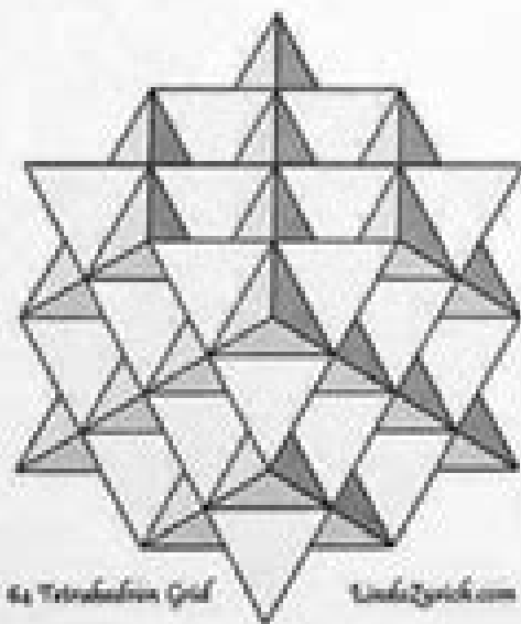
64 Tetrahedron
