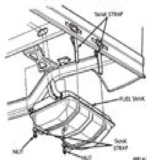
Fig. 3 Fuel Tank Remove/Install—KJ Models
