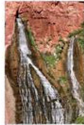
Figure 10.2 The Hydrologic Cycle: Springs and Streams
