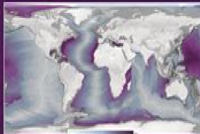
Age of Sea Floor Contours indicate 1 million years
