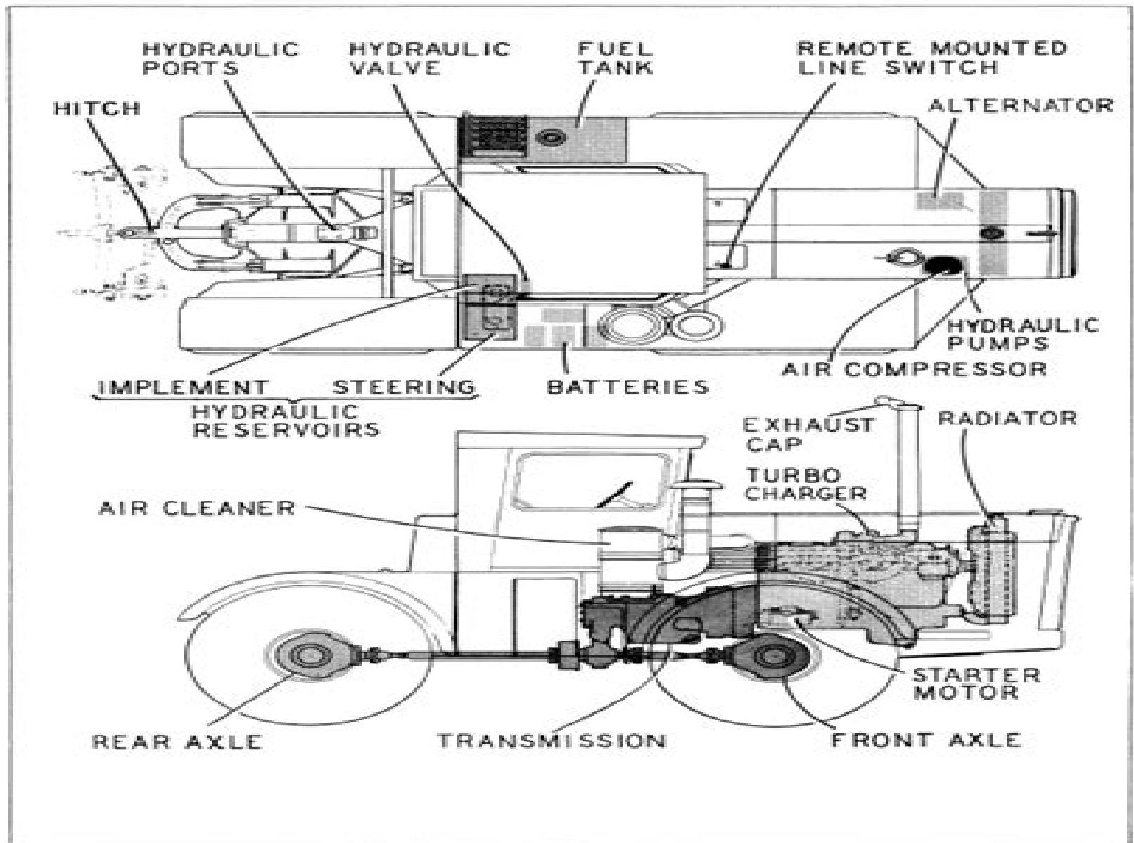
Figure 5. General arrangement
