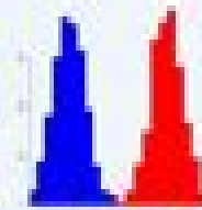
Surface Crystallinity
