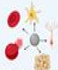
Particle Size/Shape
