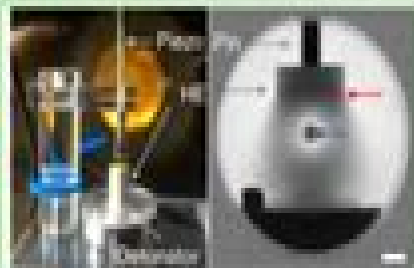
Detonation Nanodiamonds
