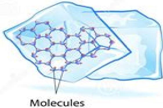
MATTER
