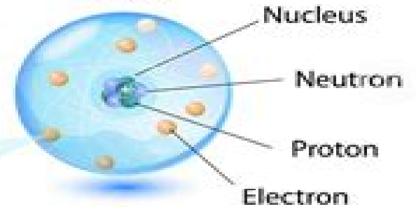
ATOM
