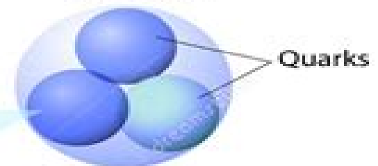
NEUTRON
