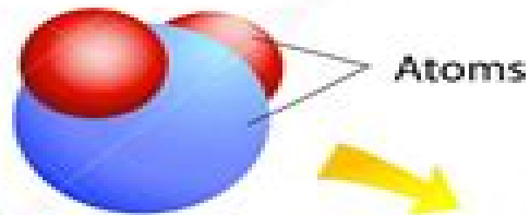
MOLECULE
